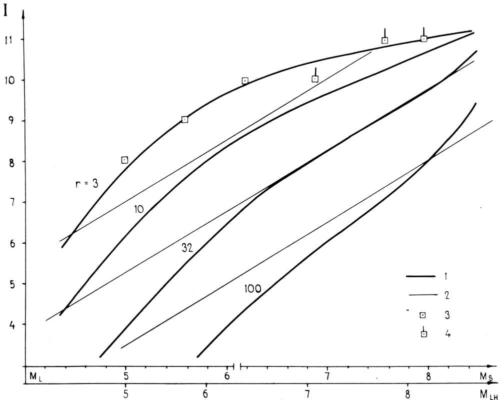
Figure 5. Calculated relation between intensity I (MSK) and magnitude for distances 3, 10, 32 and 100 km from the source centre. The level of calculated curves is selected for the best fit with the empirical relation. (1) Calculated curves. (2) Empirical relation according to Shebalin (1976). (3) and (4) Upper limits of intensity and lower bound of upper limit of intensity in epicentral zone according to Shebalin (1974).
